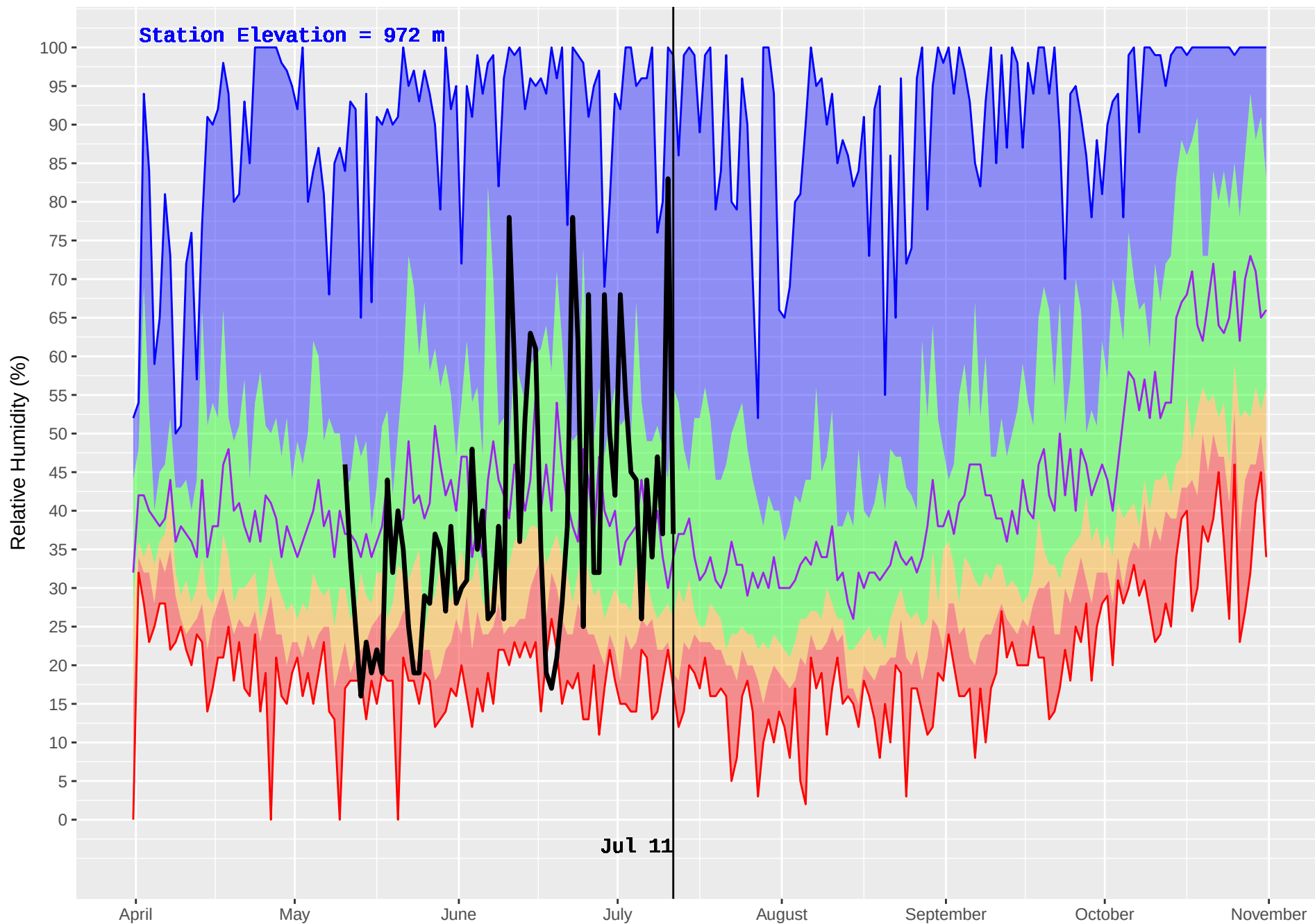
SPARKS LAKE (305) : Historical (1991–2016) and Current (2018) Noon Relative Humidity
