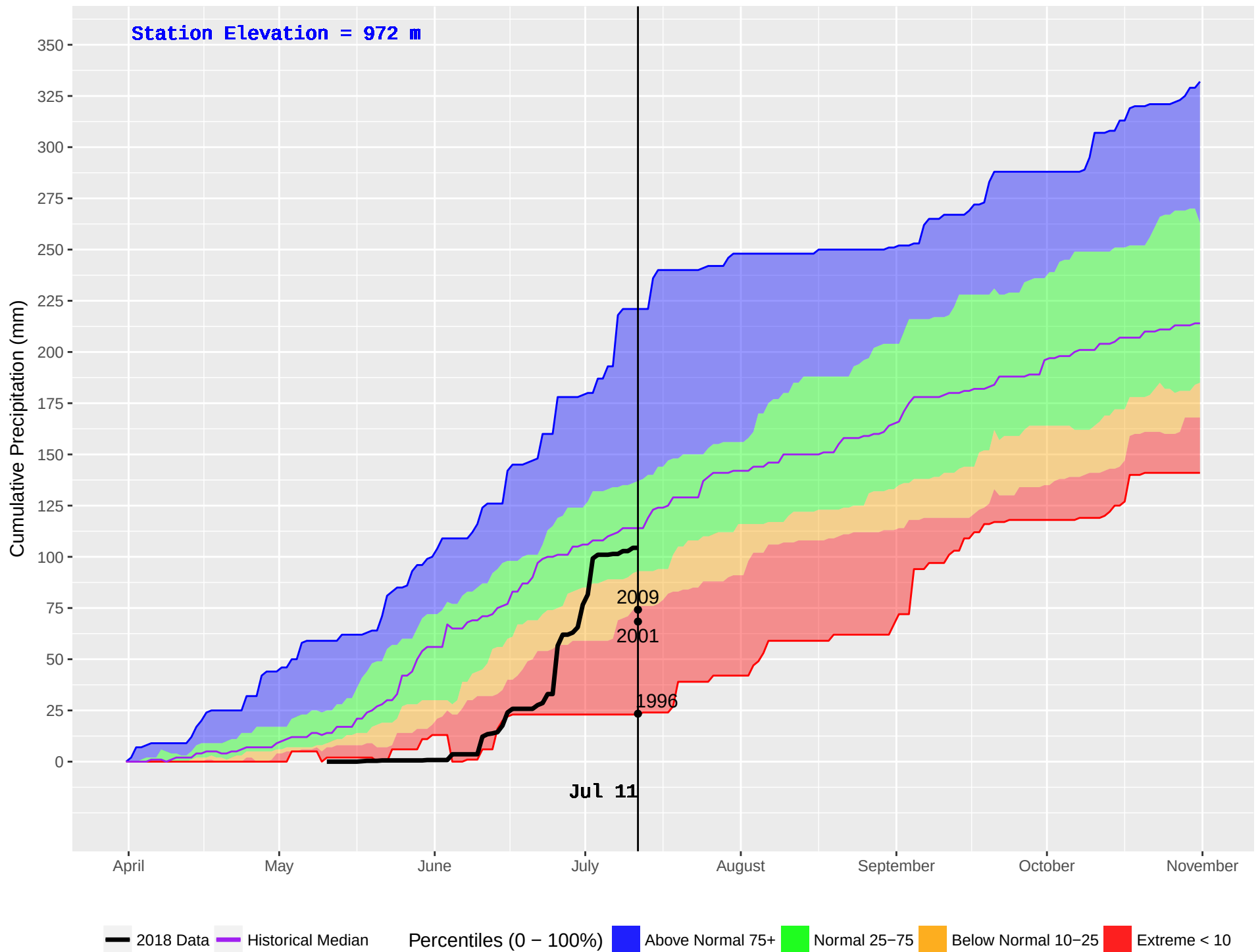
SPARKS LAKE (305) : Historical (1991–2016) and Current (2018) Noon Cumulative Precipitation
