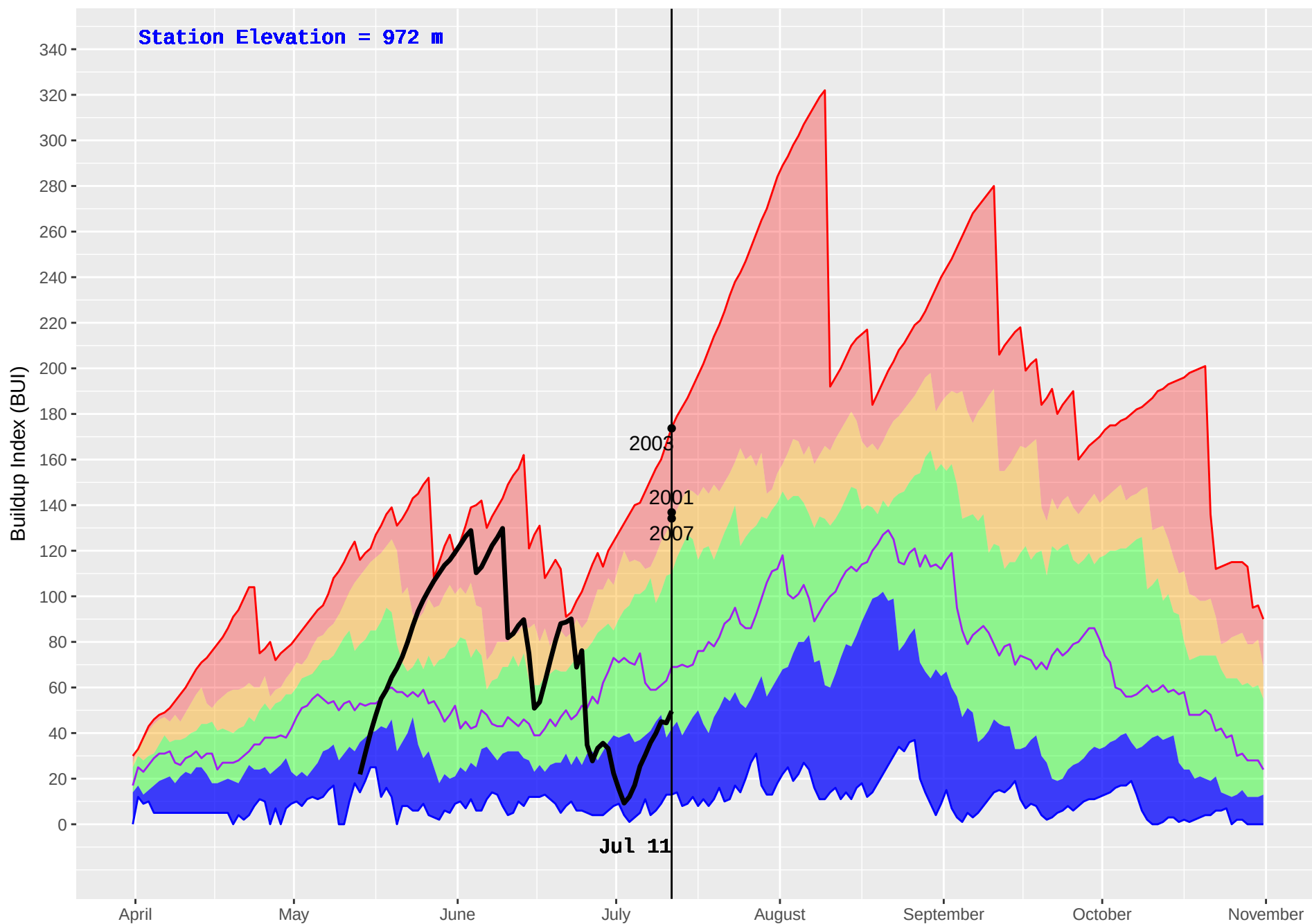
SPARKS LAKE (305) : Historical (1991–2016) and Current (2018) Noon Buildup Index (BUI)
