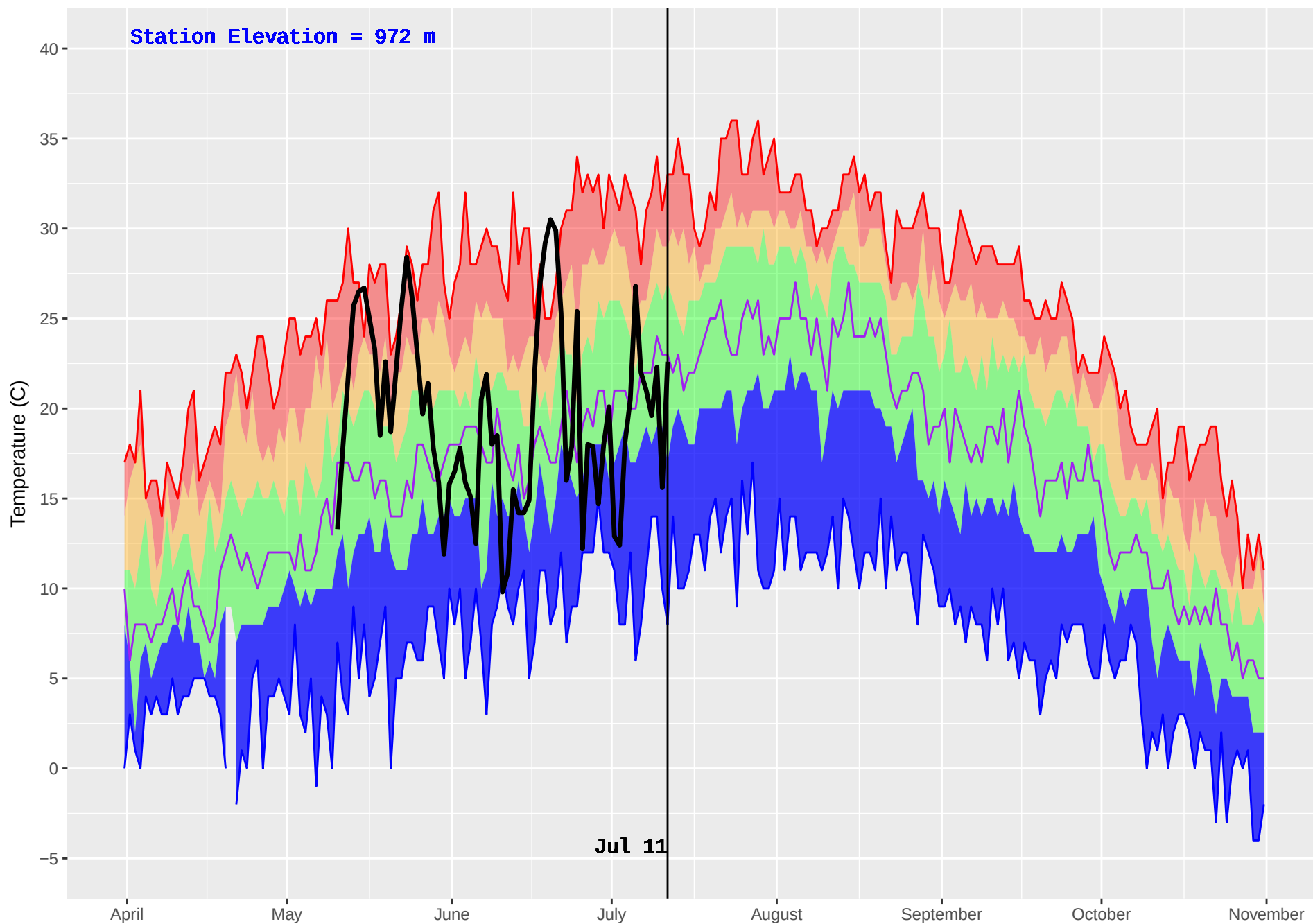
SPARKS LAKE (305) : Historical (1991–2016) and Current (2018) Noon Temperature
